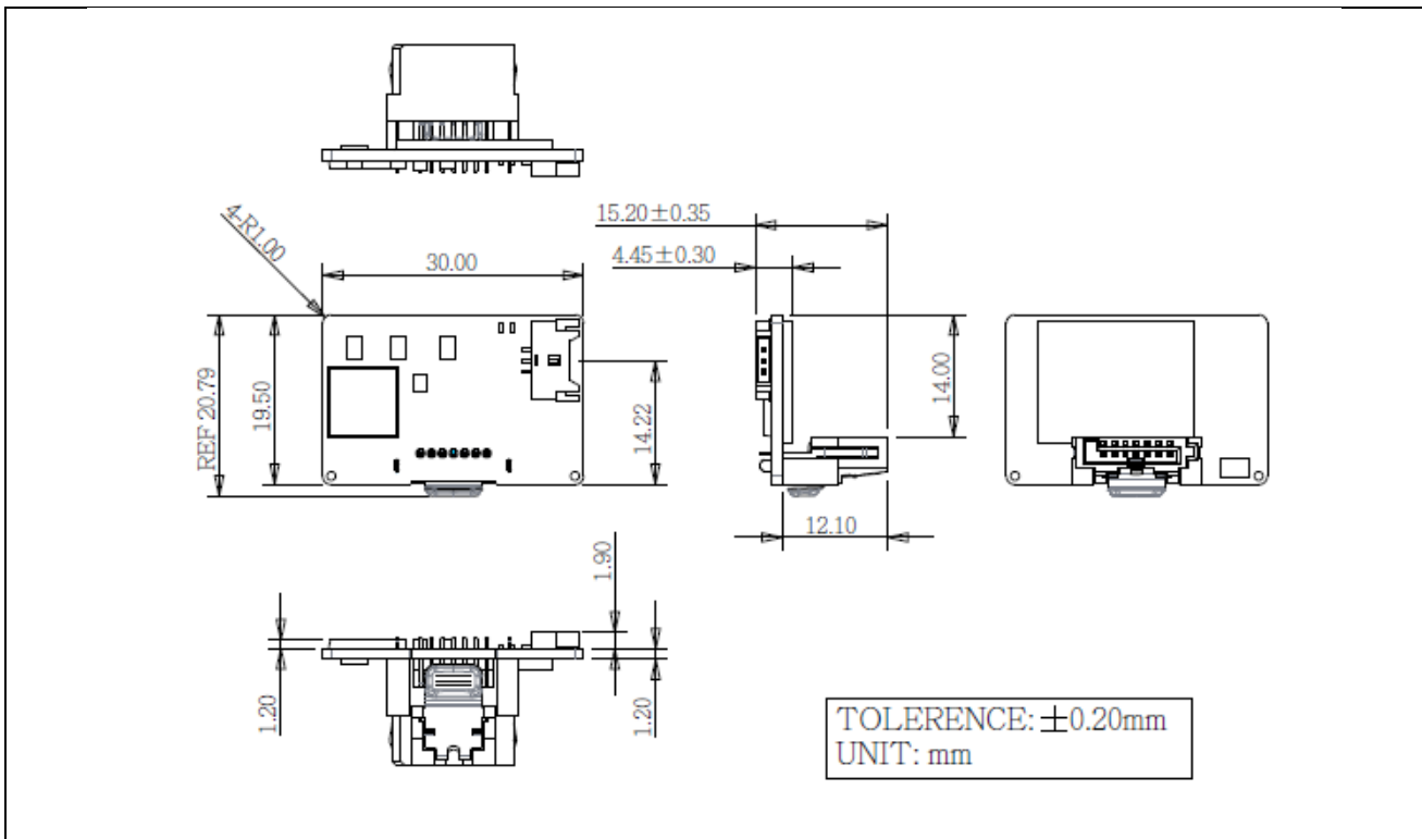
Figure 2: Innodisk SATADOM-SH Type D 3SE4 mechanical diagram
