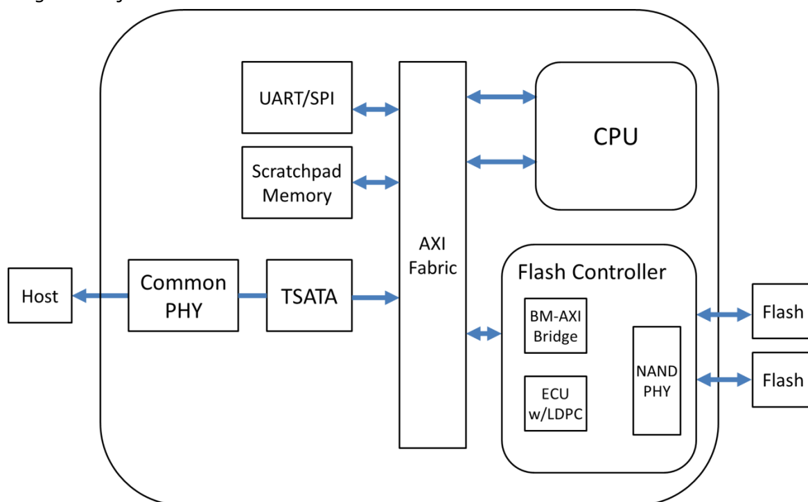
Figure 3: Innodisk SATADOM-SH Type D 3SE4 Block Diagram
