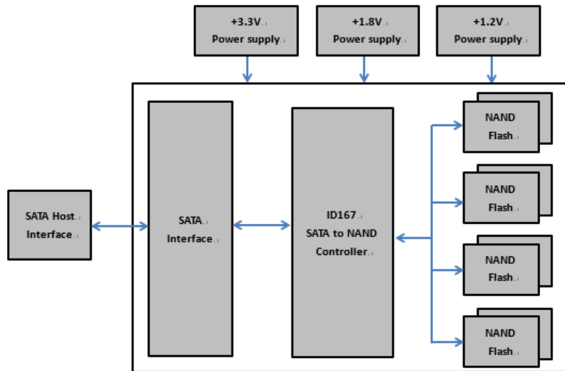
Figure 2: Innodisk SERVERDOM-H 3SE Block Diagram
