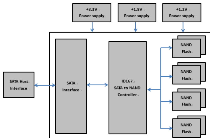
Figure 2: Innodisk SERVERDOM-V 3SE Block Diagram
