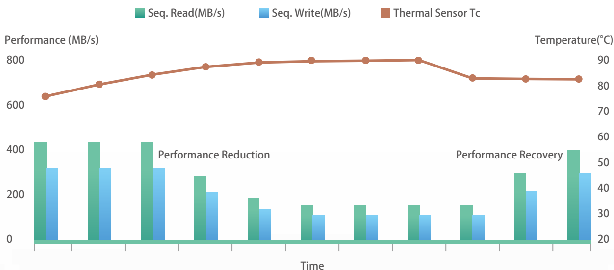
Read/Write Performance vs Temperature
