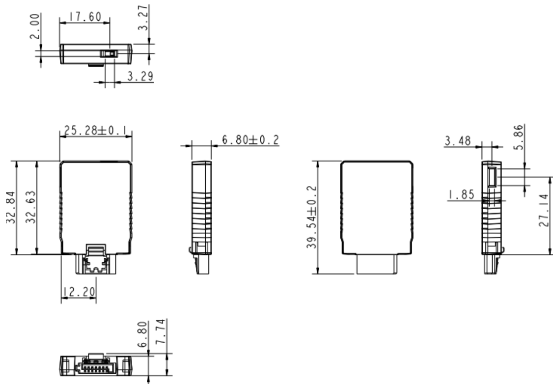
Figure 7: SATADOM D150QV (No Hook) mechanical dimensions
