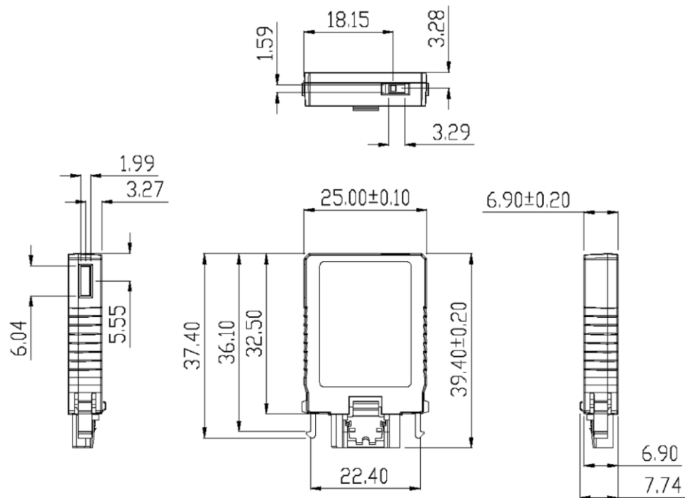
Figure 6: SATADOM D150QV mechanical dimensions
