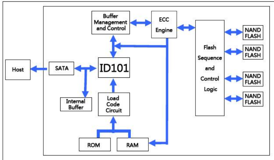
Figure 2: InnoDisk SATADOM D150QV Block Diagram
