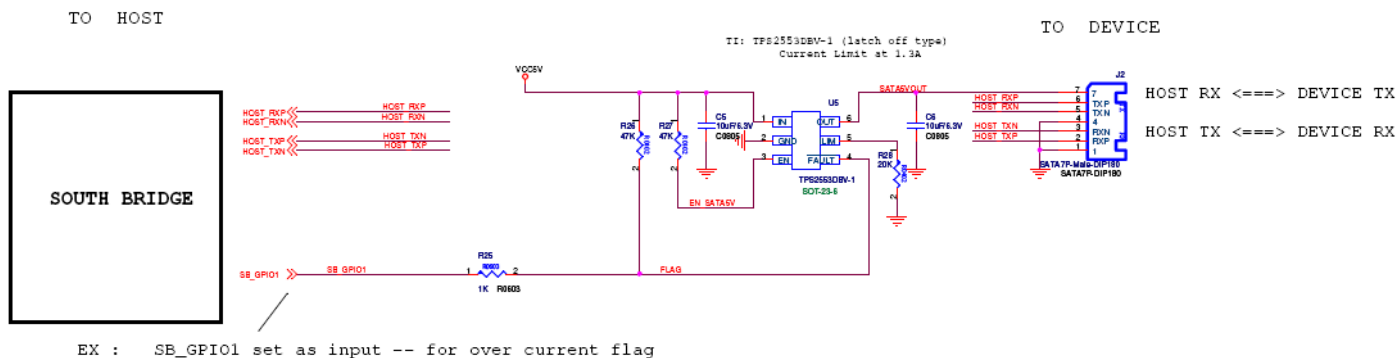
Figure 5: Fuse circuit design for SATADOM D150QV series with Pin7 VCC
