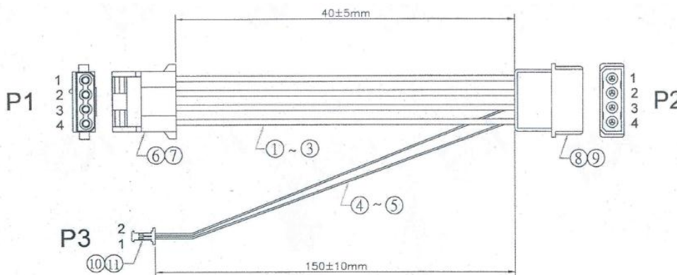
Figure 8: SATADOM D150QV power cable mechanical drawing
