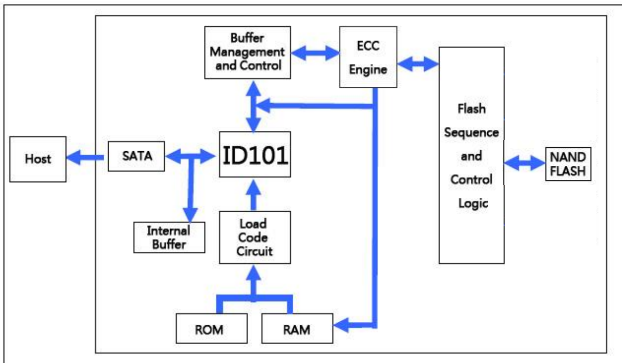
Figure 2: Innodisk SATADOM D150SH-L Block Diagram
