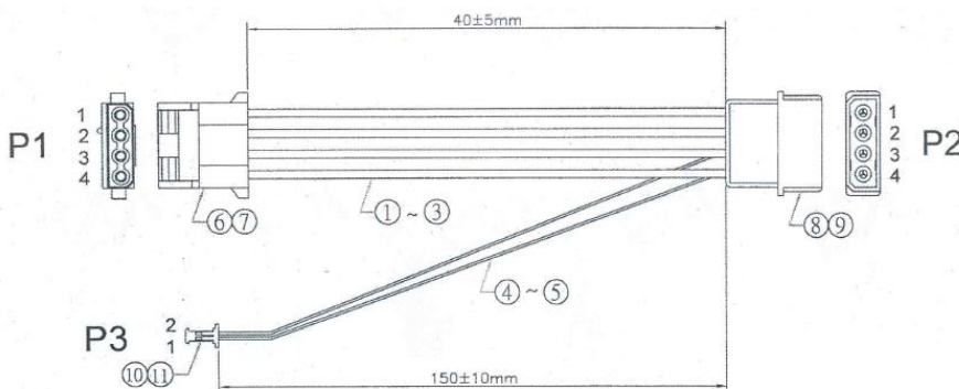
Figure 6: SATADOM D150SH-L power cable mechanical drawing
