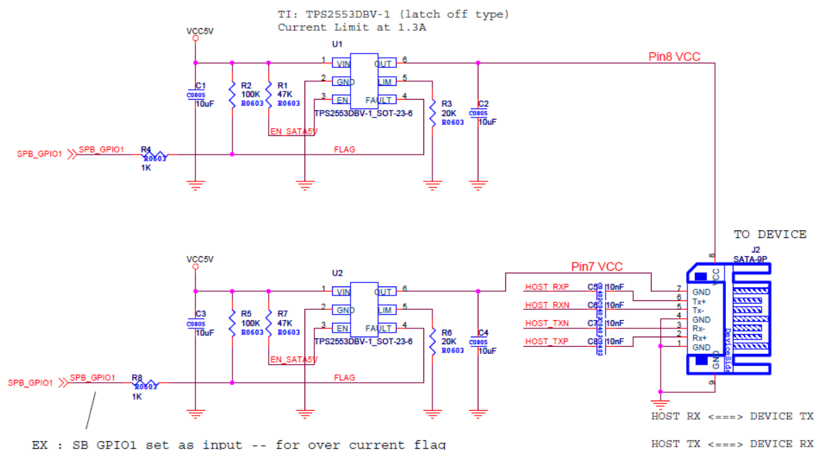
Figure 7: Pin 8 / Pin 7 host design in reference circuit
