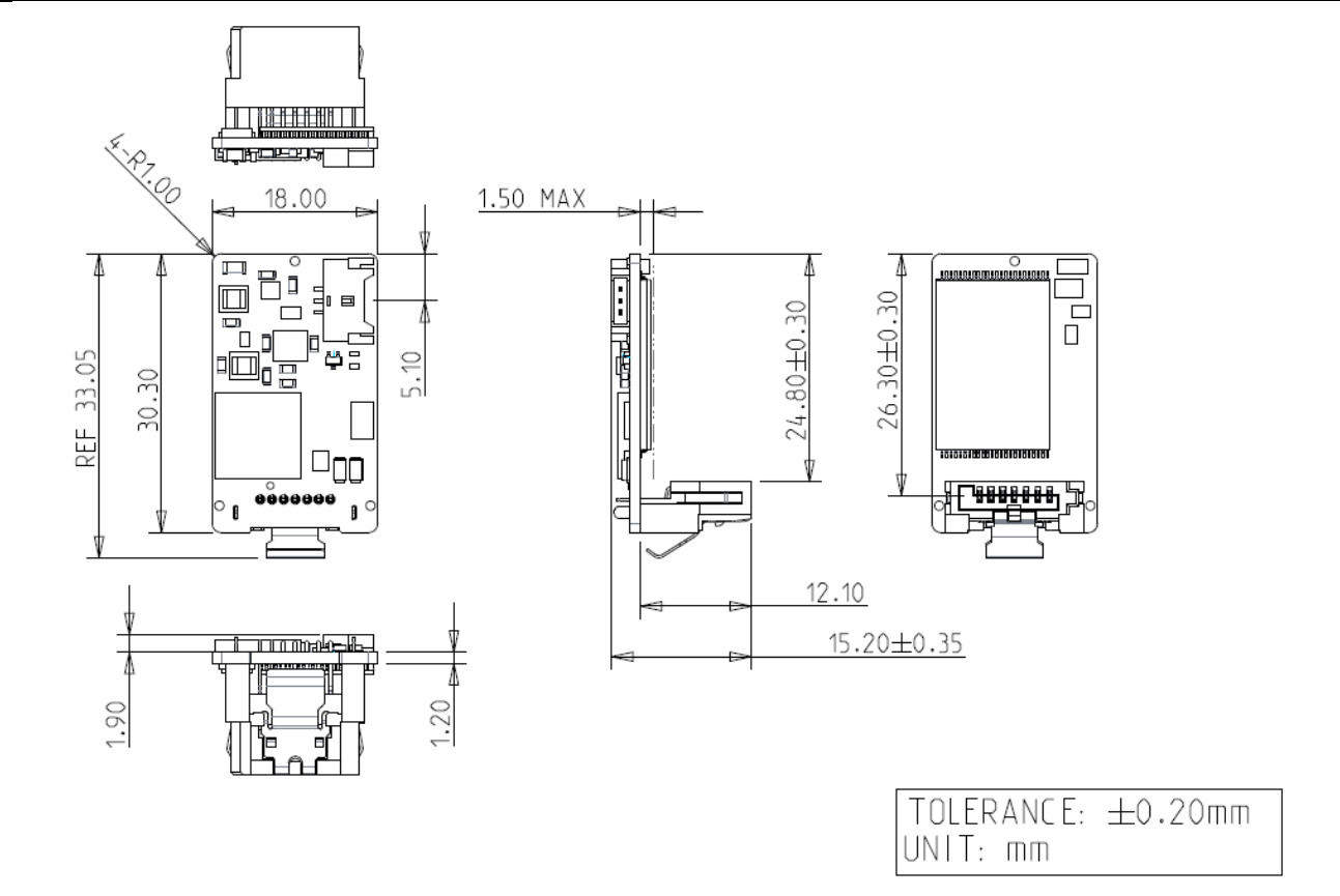
Figure 2: Innodisk SATADOM-SH 3TE7 (TSOP) mechanical diagram
