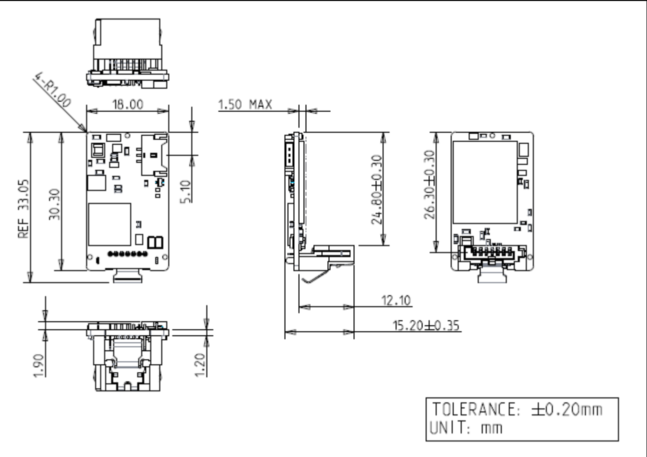
Figure 3: Innodisk SATADOM-SH 3TE7 (BGA) mechanical diagram
