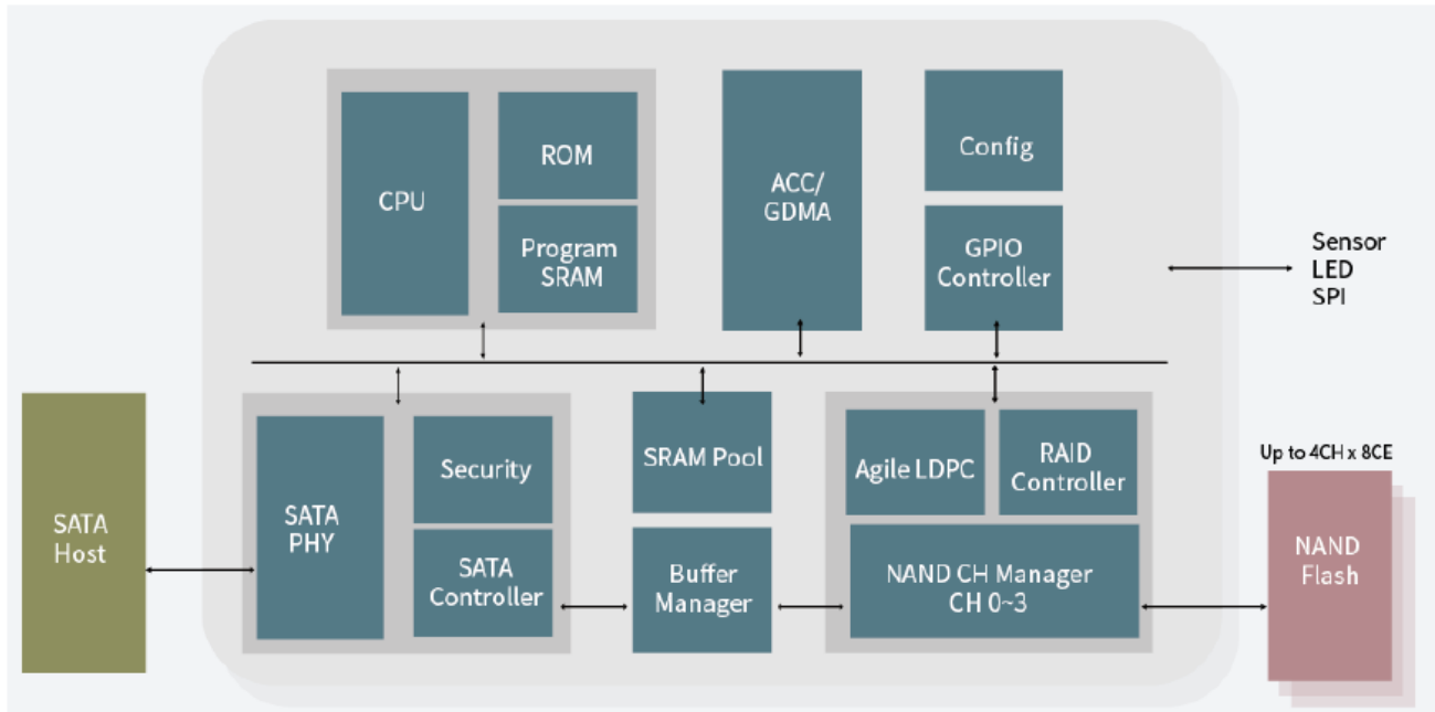
Figure 4: Innodisk SATADOM-SH 3TE7 Block Diagram
