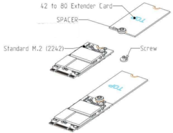
Extender Board Use Case
