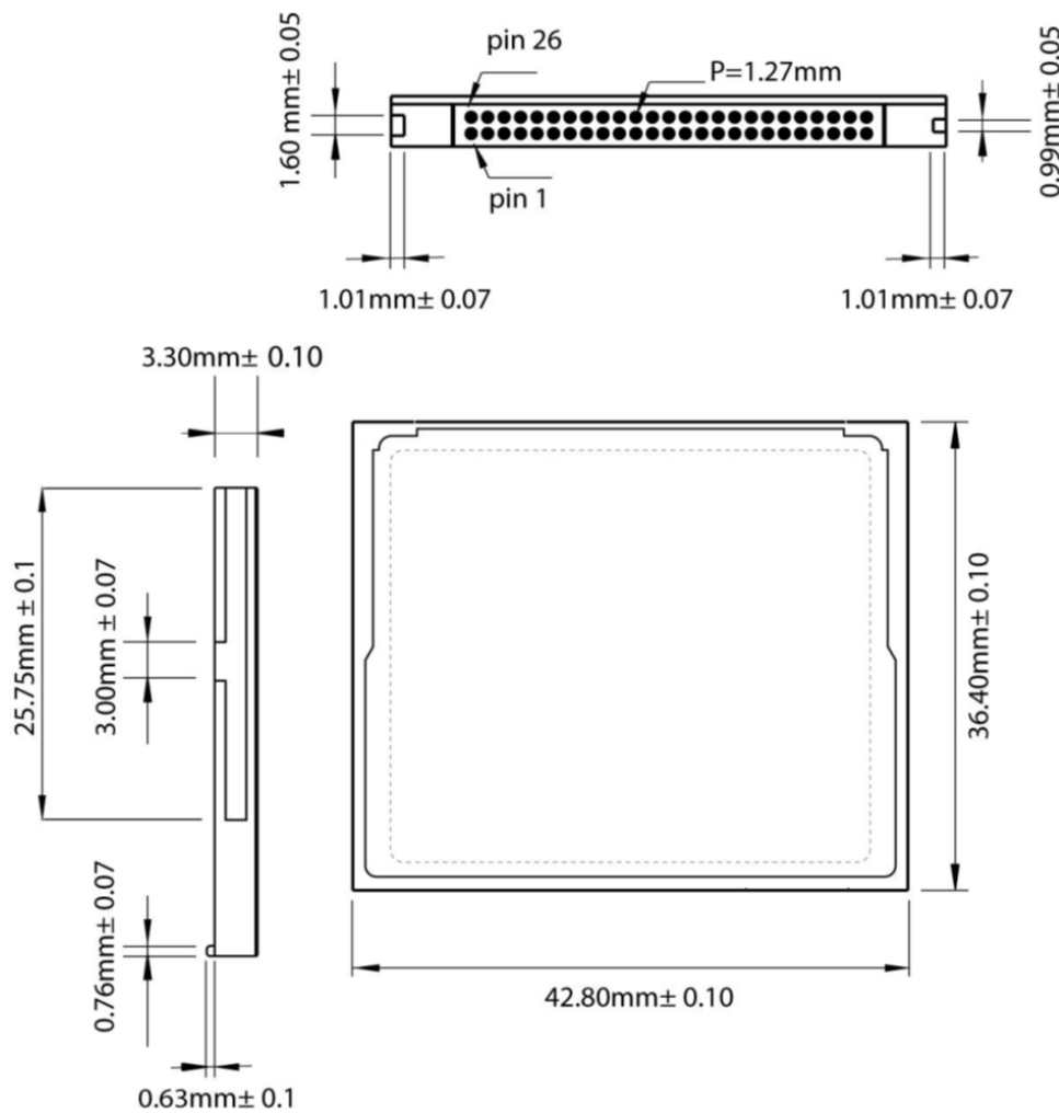
Figure 2 Mechanical Dimension of iCF 1ME2
