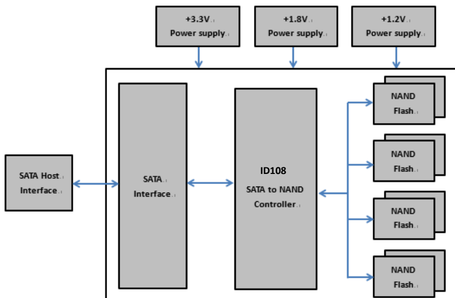
Figure 2: Innodisk ServerDOM-L 3ME3 Block Diagram
