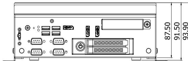
Rear View
