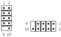
USB 2.0 Header
