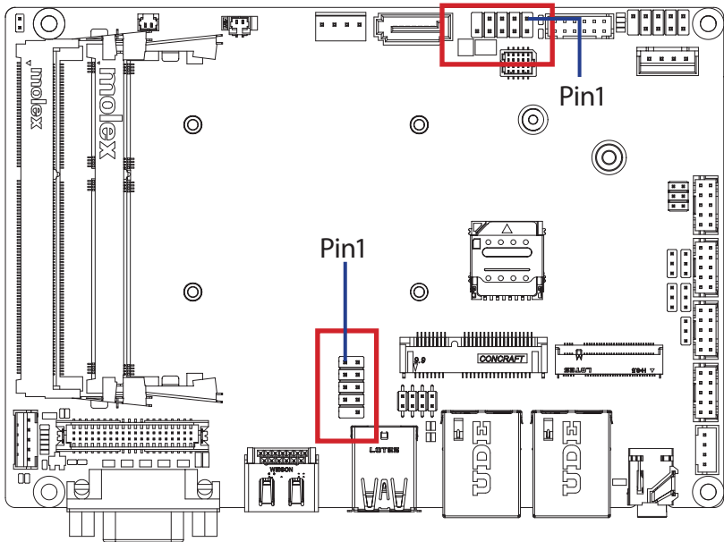
USB 2.0 Header
