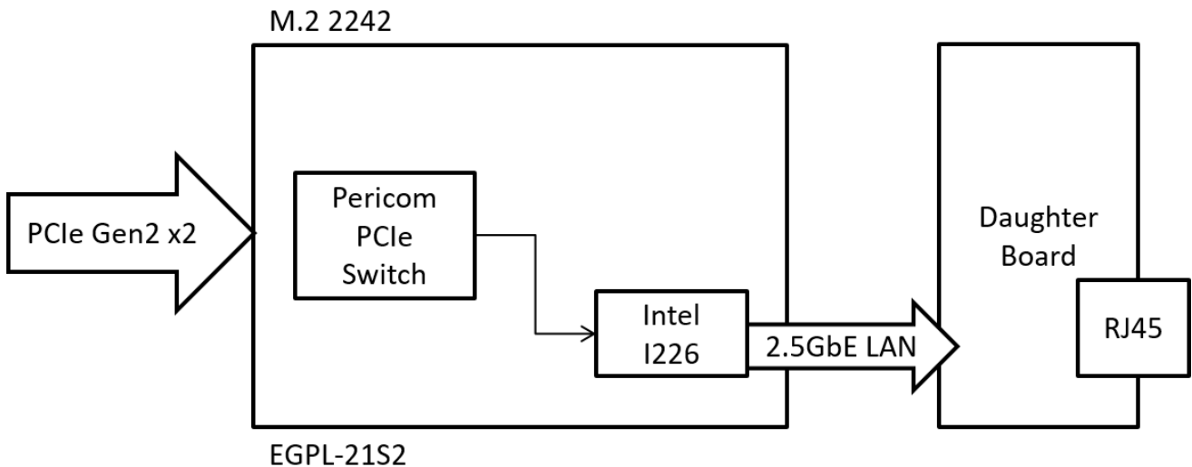
Figure 1: Block Diagram
