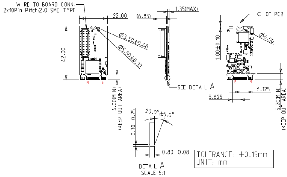
Figure 6: EGPL-21S2 M.2 Board Drawing
