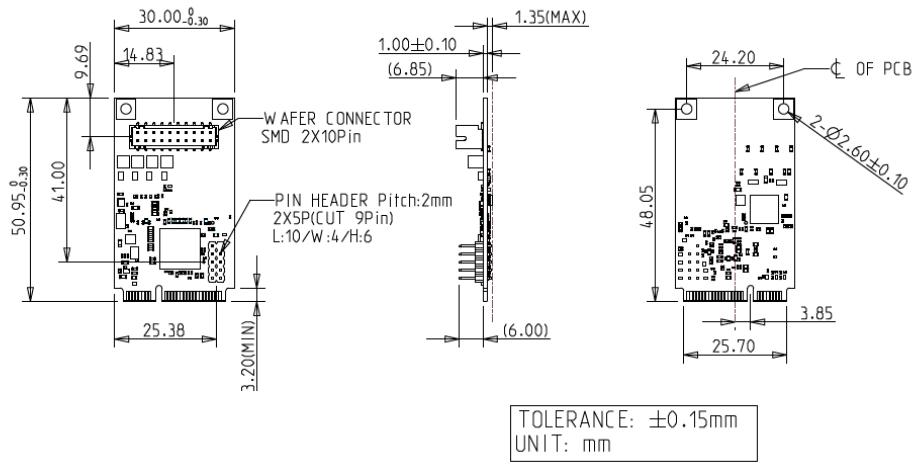
Figure 5: EMPL-G1N1 mPCIe Board Drawing
