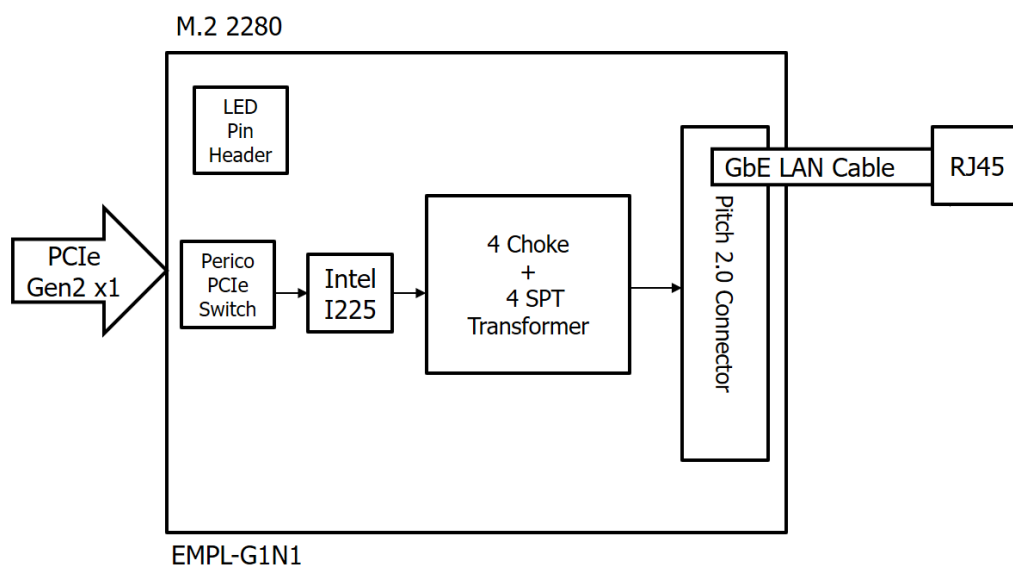
Figure 1: Block Diagram
