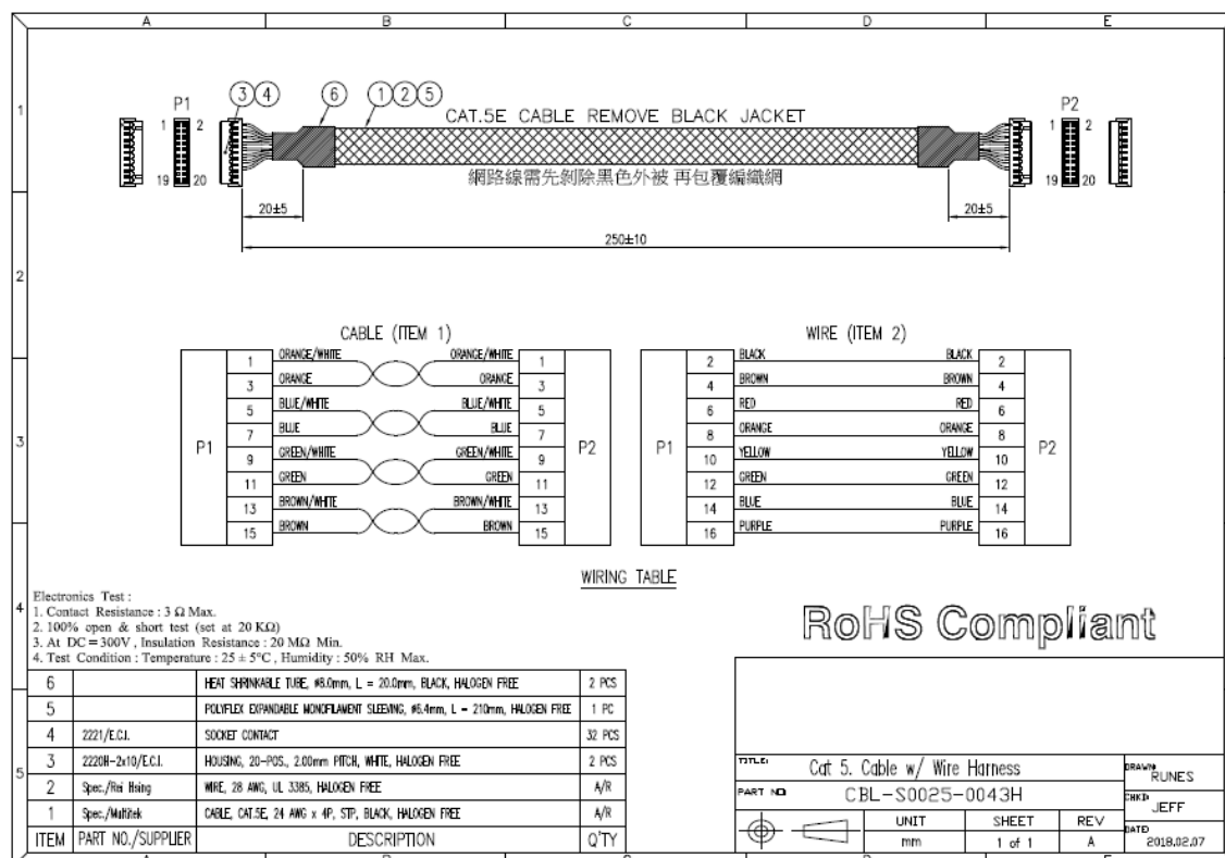
Figure 11: Board to Board LAN Cable Drawing
