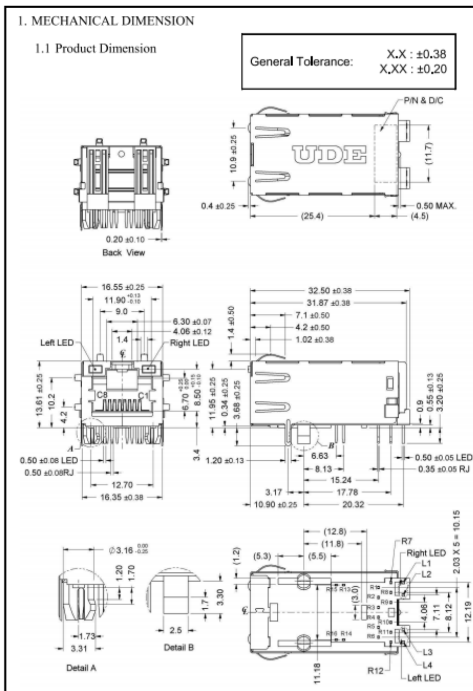
Figure 6: RJ45 Connector Drawing
