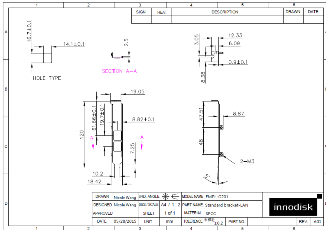
Figure 10: Bracket Drawing
