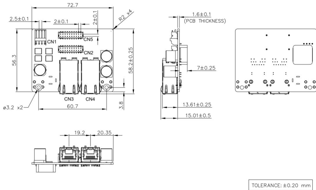
Figure 9: Bracket Daughter Board Drawing - 4Pin Header (EMPL-G2P2-C2/W2)
