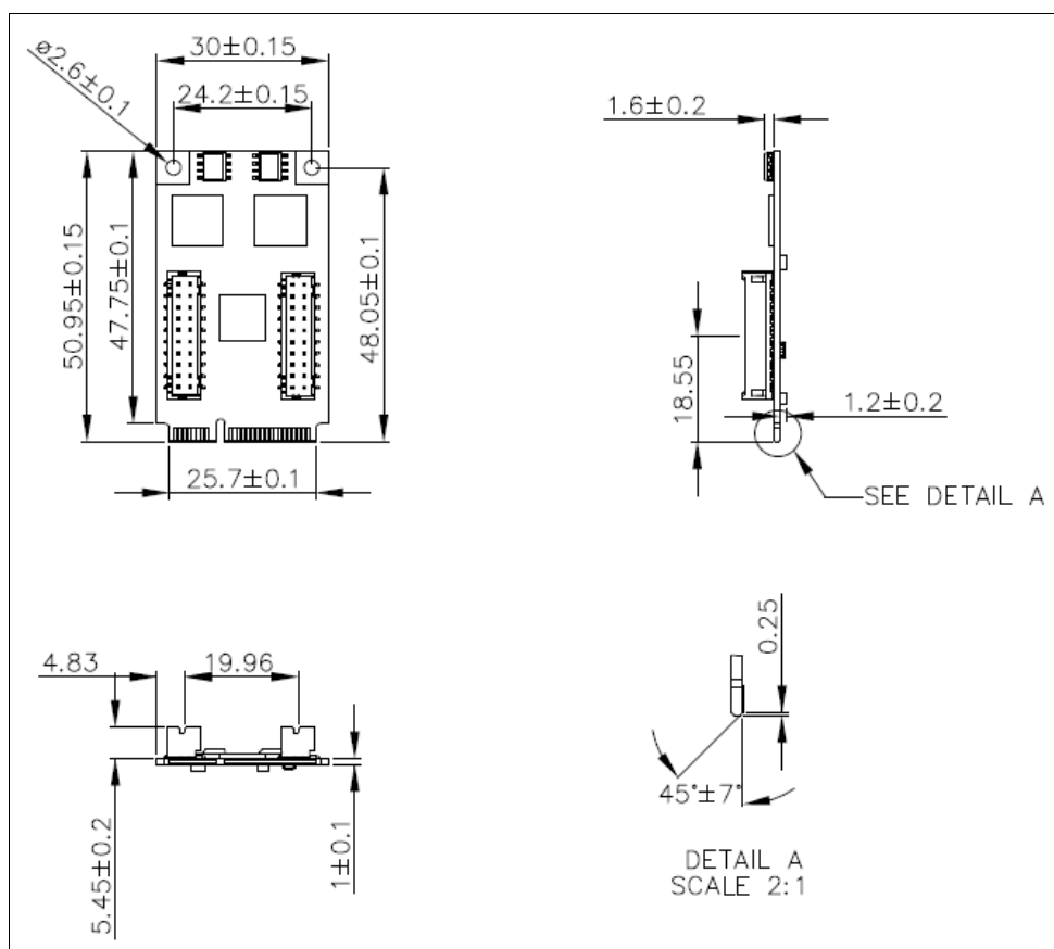
Figure 7: EMPL-G2P2 mPCIe Board Drawing
