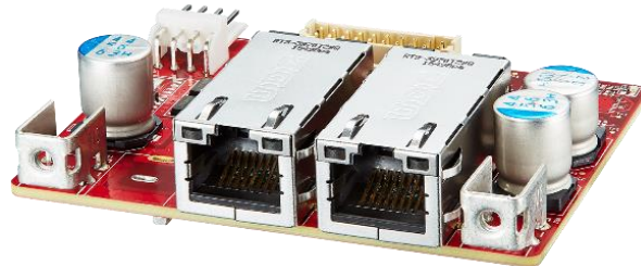
Figure 3: Mounting Hole, 4Pin Header, Daughter Board Picture (EMPL-G2P2-C1/W1)
