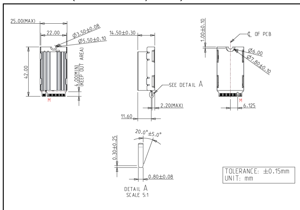
Figure 4: Innodisk M.2 (P42) 4IE3 with heatsink
