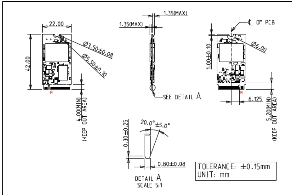
Figure 3: Innodisk M.2 (P42) 4IE3
