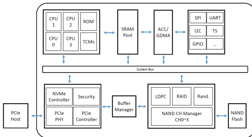
Figure 5: Innodisk M.2 (P42) 4IE3 Block Diagram
