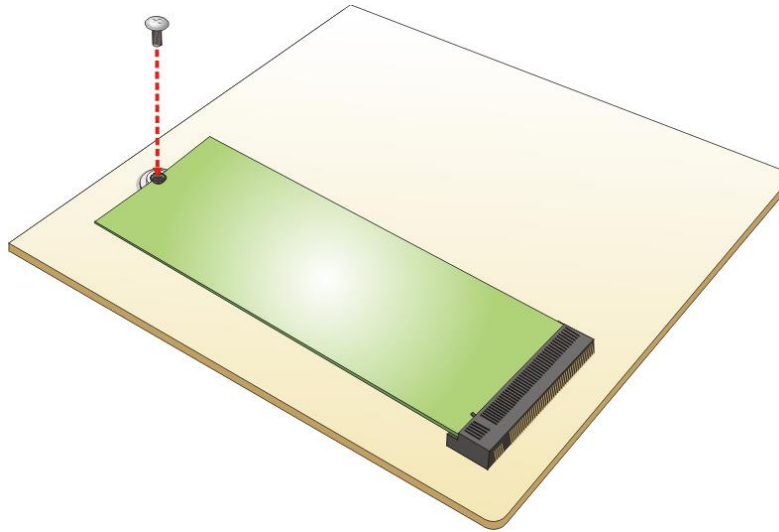
Figure 4-3: Securing the M.2 Module
