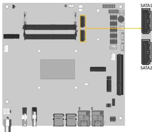
Figure 3-19: SATA 6Gb/s Drive Connectors Locations
