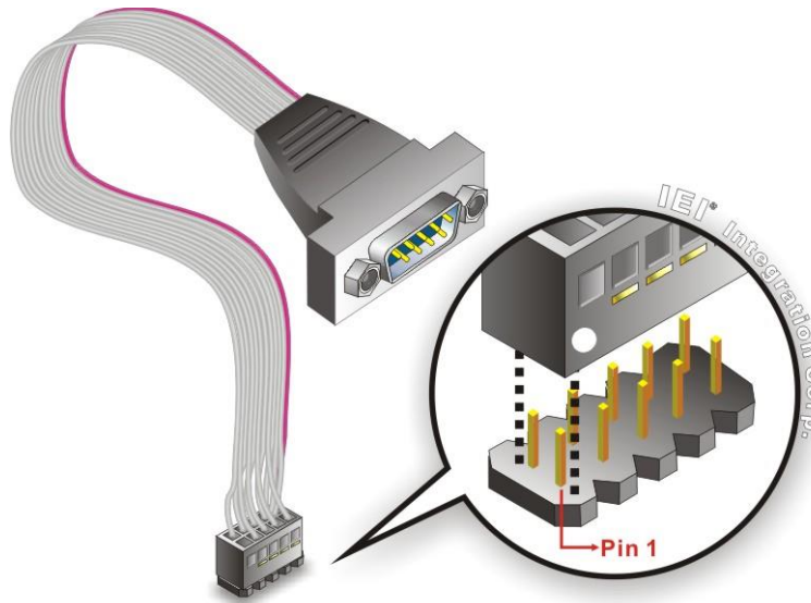
Figure 4-7: Single RS-232 Cable Installation
