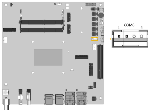
Figure 3-18: Serial Port Connector Location
