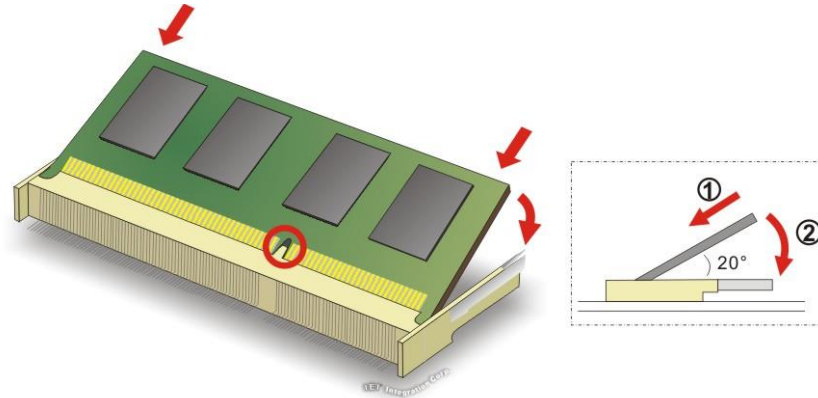
Figure 4-1: SO-DIMM Installation
