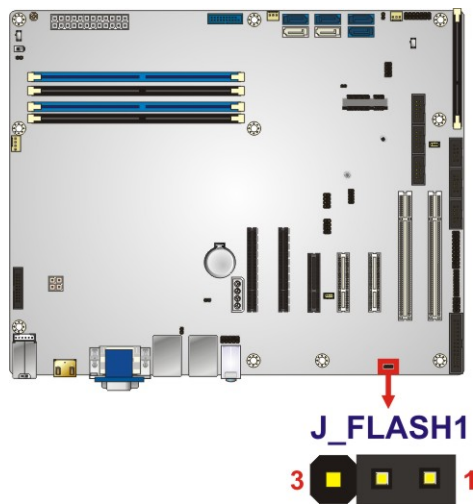
Figure 4-19: Flash Descriptor Security Override Jumper Location
