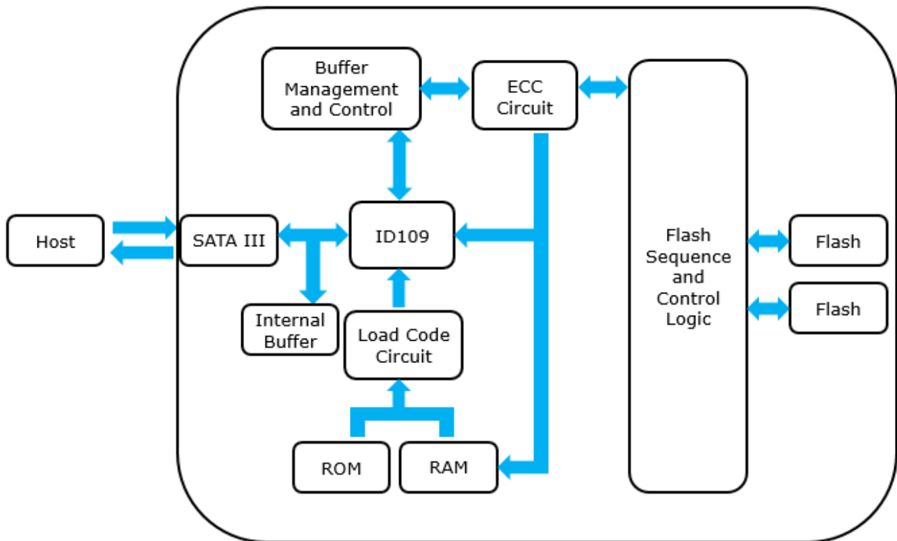
Figure 2: Innodisk SATADOM-SL 3IE3 V2 Block Diagram
