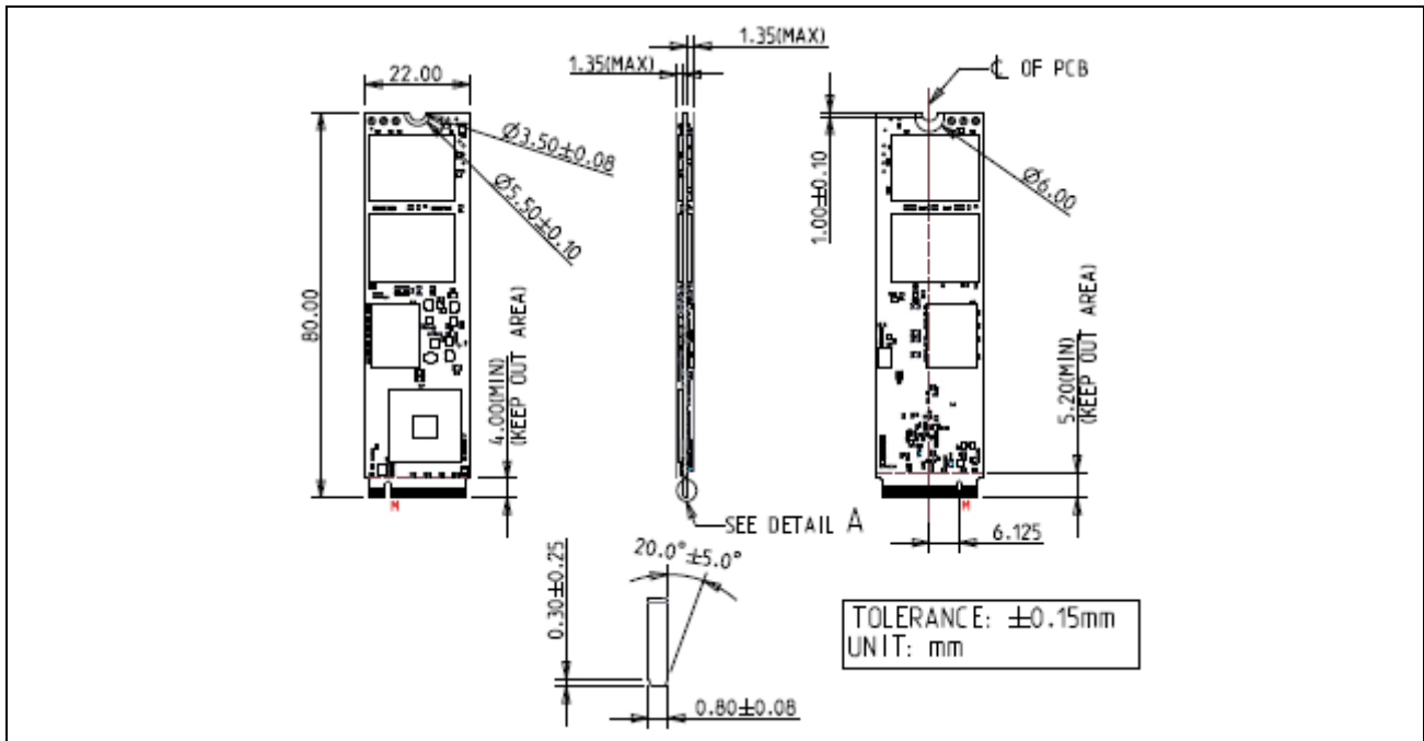
Figure 5: Innodisk M.2 (P80) 4TG2-P
