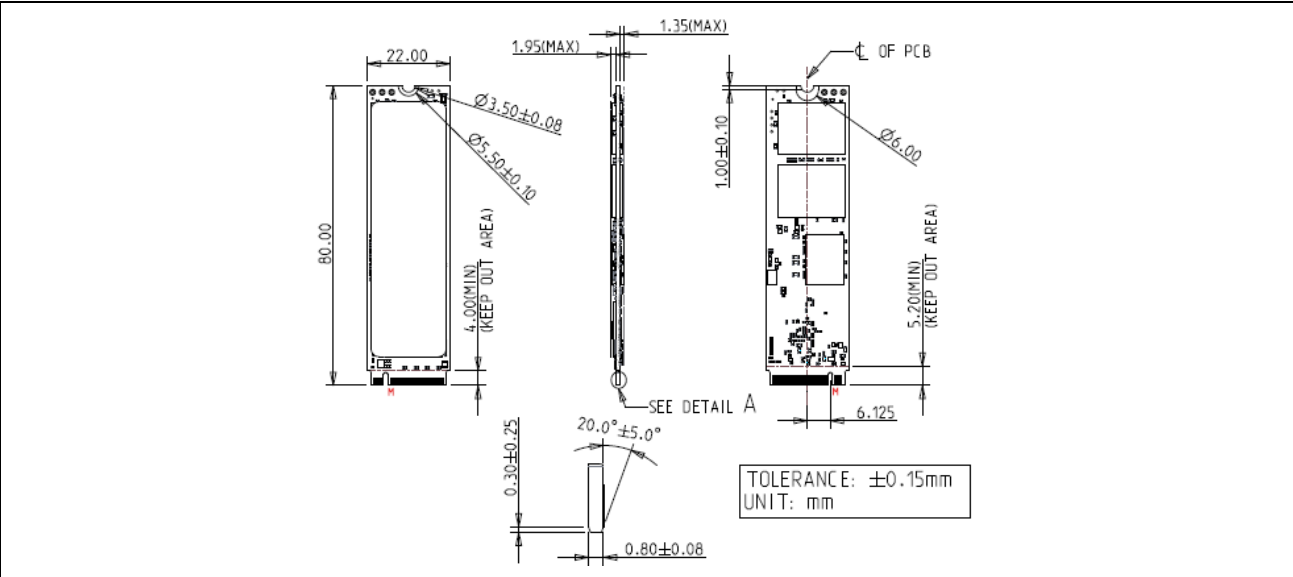
Figure 3: Innodisk M.2 (P80) 4TG2-P with heat-spreading copper layer diagram
