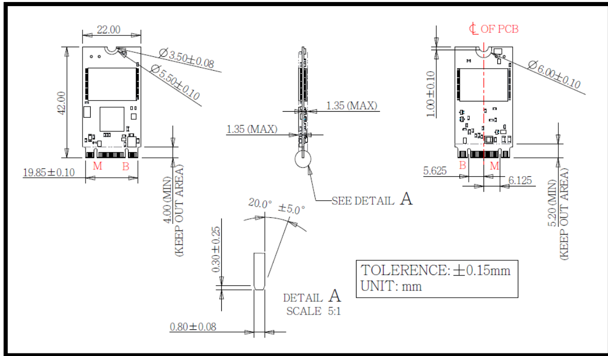
Figure 2: Innodisk M.2 (S42) 3IE7 diagram (TSOP)
