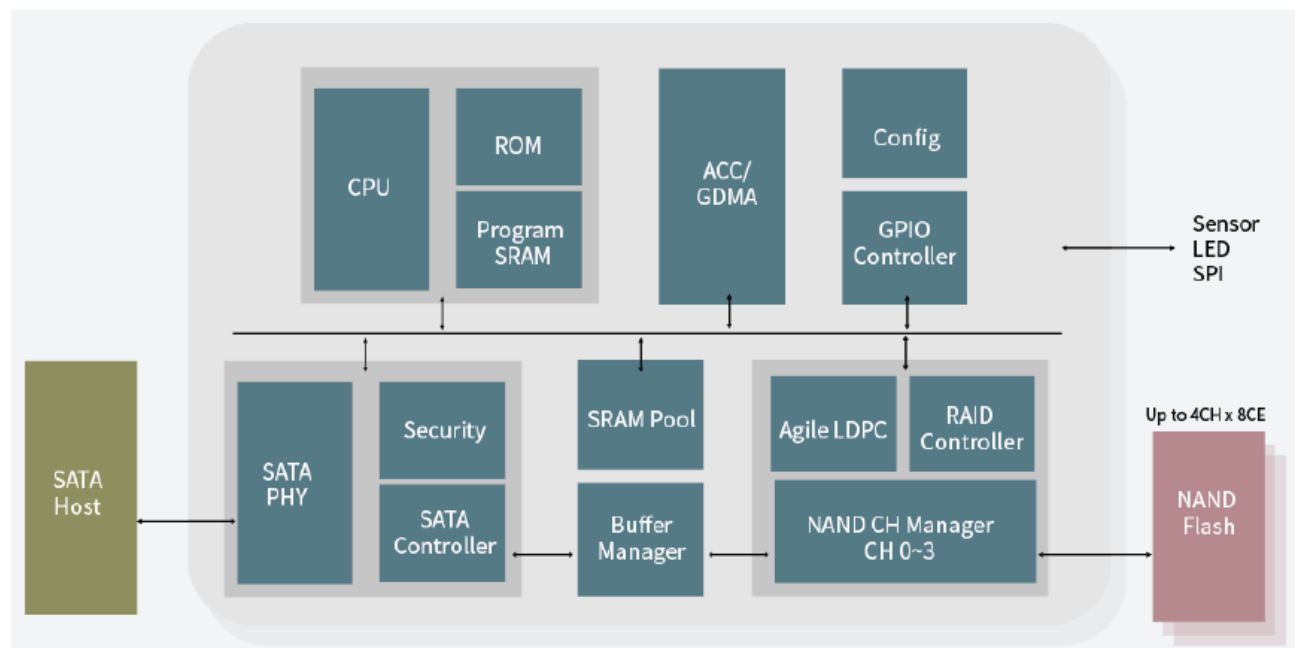
Figure 4: Innodisk M.2 (S42) 3IE7 Block Diagram
