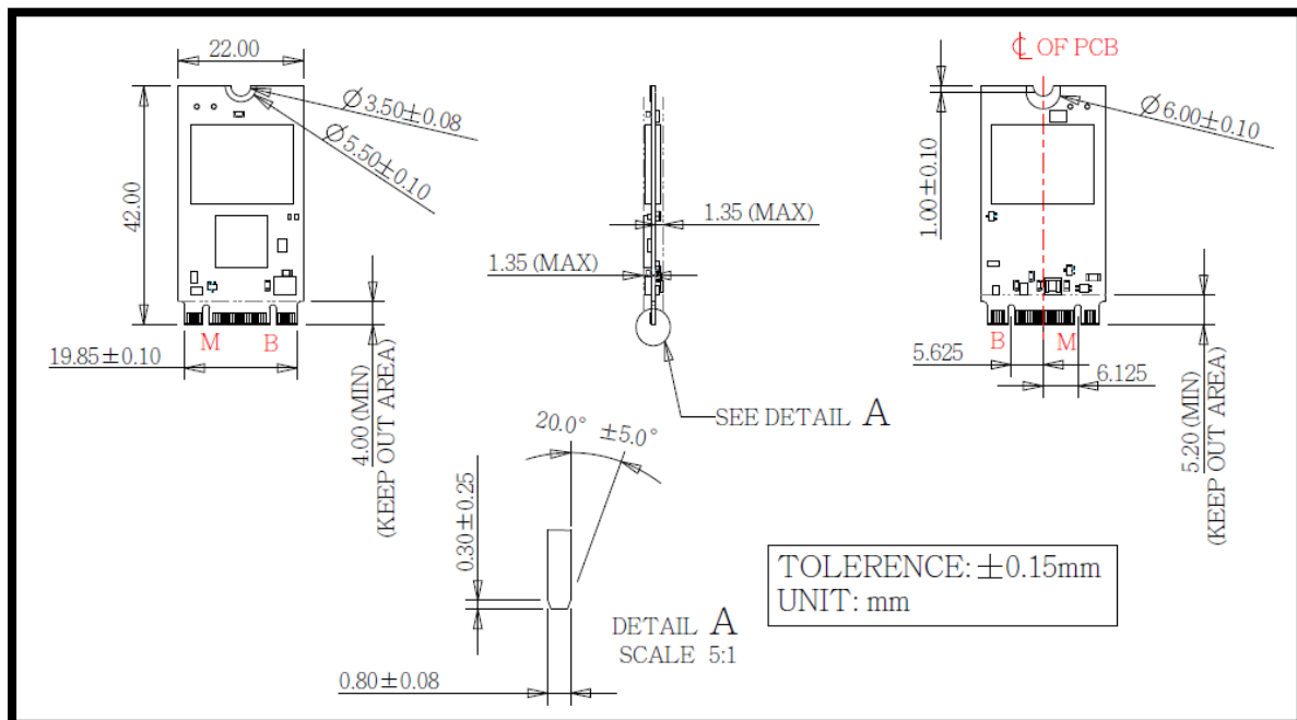
Figure 3: Innodisk M.2 (S42) 3IE7 diagram (BGA)
