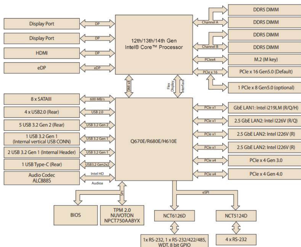
Figure 1.3 AIMB-588 B1 Block Diagram
