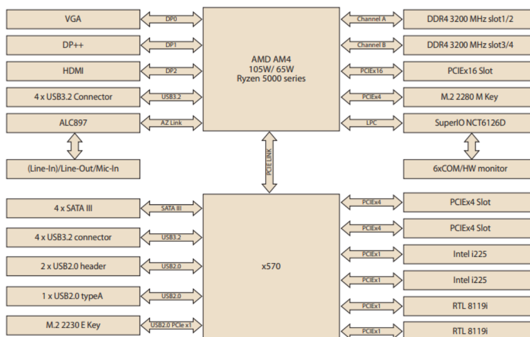
Figure 1.2 AIMB-522 Block Diagram
