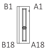
PCIe x1 connector
