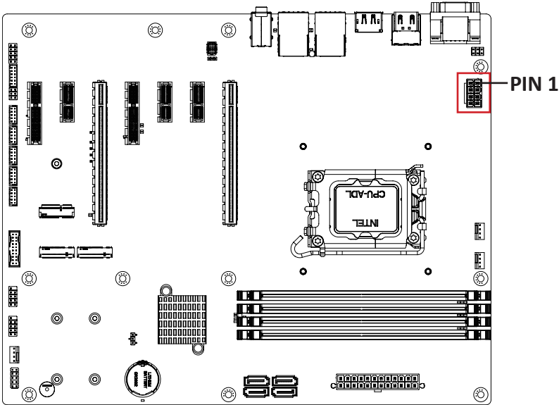
ATX 12V Connector
