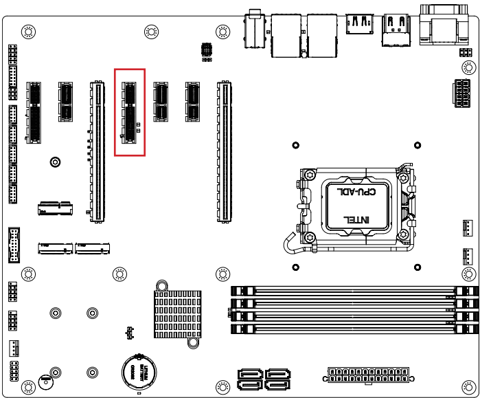
PCIe x4 connector
