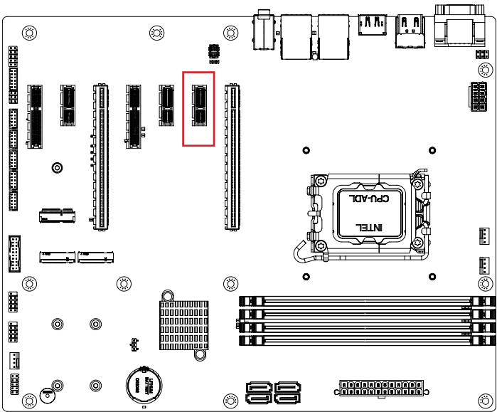
PCIe x1 connector
