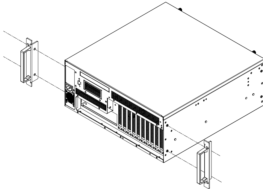
Figure 2.18 Attaching the Ears and Handles/ 安裝耳柄
