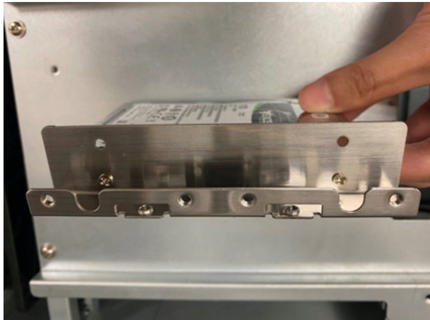
Figure 2.13 Attach 2.5" HDD with bracket/ 鎖附 2.5" 硬盘与支架 / 鎖附 2.5" 硬碟與支架
