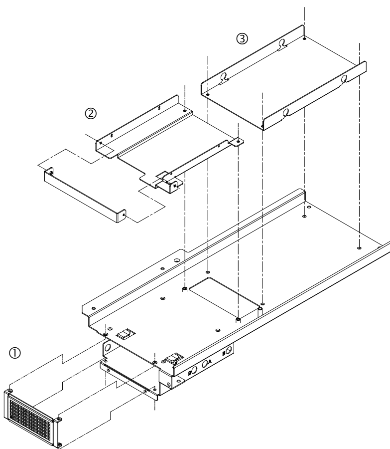
Figure 2.6 Remove Screws and Brackets/ 移除螺丝与对应支架 / 移除螺絲與對應支架
