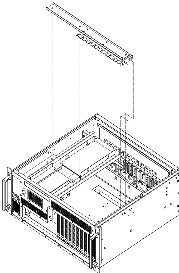
Figure 2.4 Remove Hold-on Bar/ 移除檔杆 / 移除檔桿
