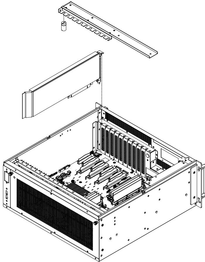
Figure 2.21 PCIe Cards assembly/ 扩充卡安装 / 擴充卡安裝
