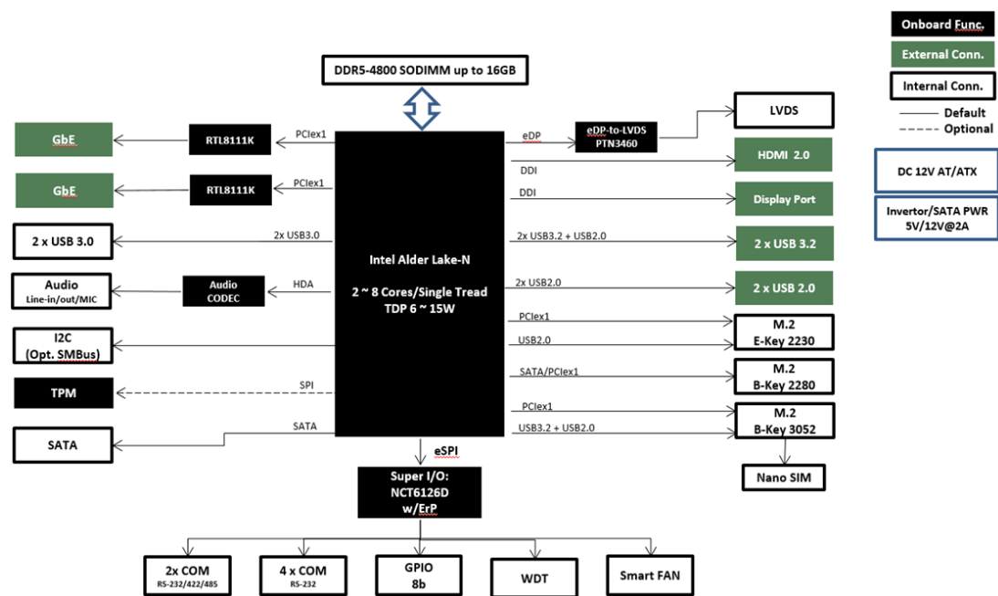
Figure 1.1 Block Diagram
