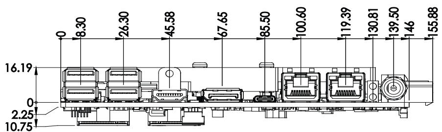
Figure 2.6 MIO-5377 Mechanical Diagram (with Heatspreader)
