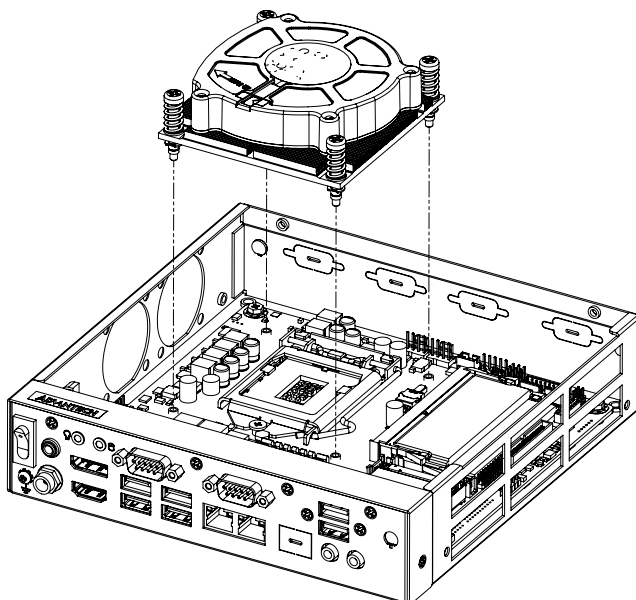
Figure 2.2 CPU Cooler installing/ 安装CPU风扇/安裝CPU風扇
