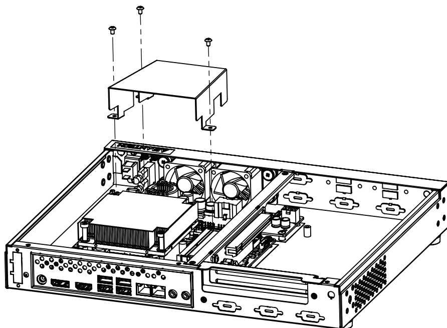
Figure 2.1 Assemble Air Duct / 组装导风罩 / 組裝導風罩
