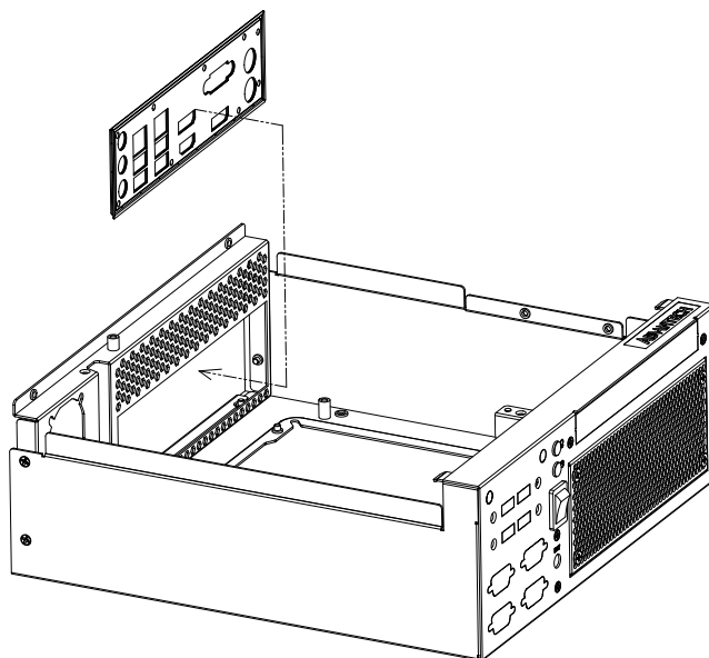
Figure 2.7 Installing IO Shielding/ 安裝 IO 挡板 / 安裝 IO 擋板
