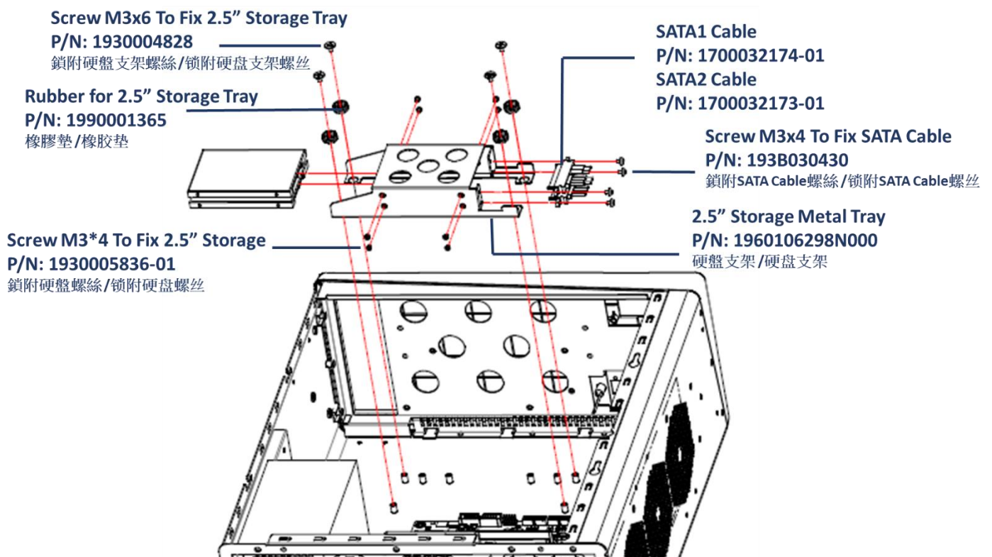
Figure 2.2 Installing Storage / 组装硬盘 / 組裝硬盤
