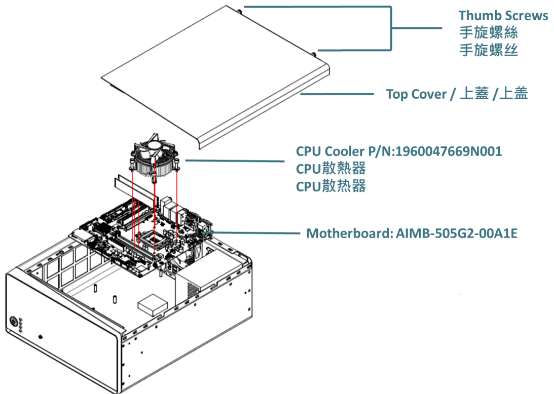
Figure 2.1 Open the Chassis Cover / 打开机箱顶盖 / 打開機箱上蓋
