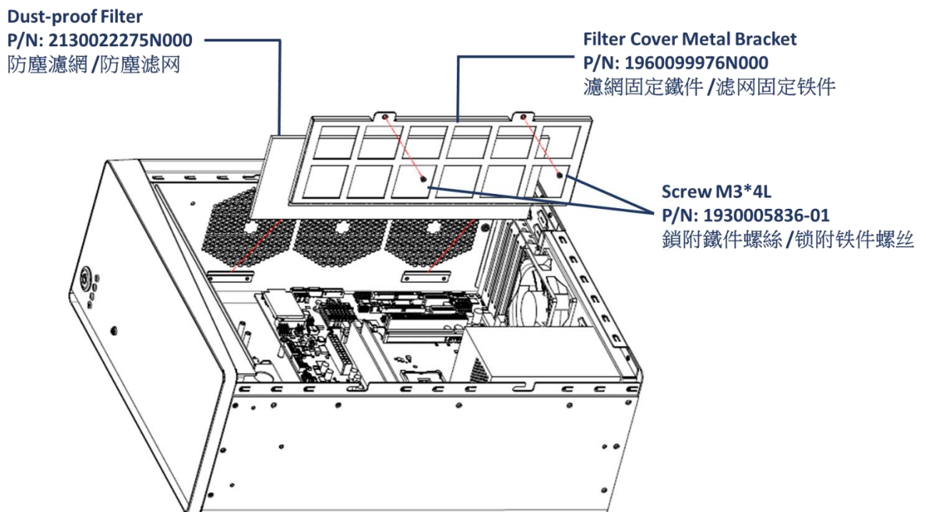
Figure 2.3.2 Dust-proof Filter Maintenance / 防尘滤网維護 / 防尘滤网维护
