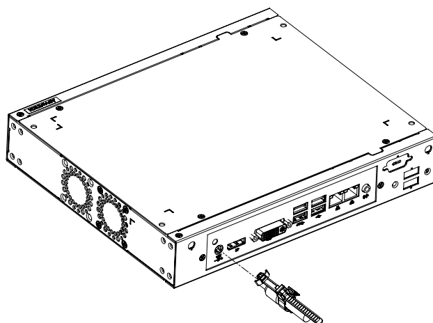
Figure 2.12 Installing the Power Cord Lock Harness/ 安裝电源线防脱落扣具 / 安裝電源線防脫落扣具
