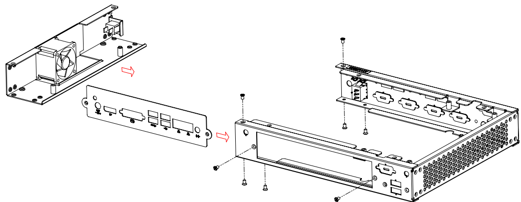
Figure 2.2 Assemble the Rear IO Panel / 組裝後面 IO 面板 / 組裝後面 IO 面板
