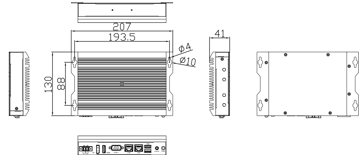
ACS-2310A Wall Mount
