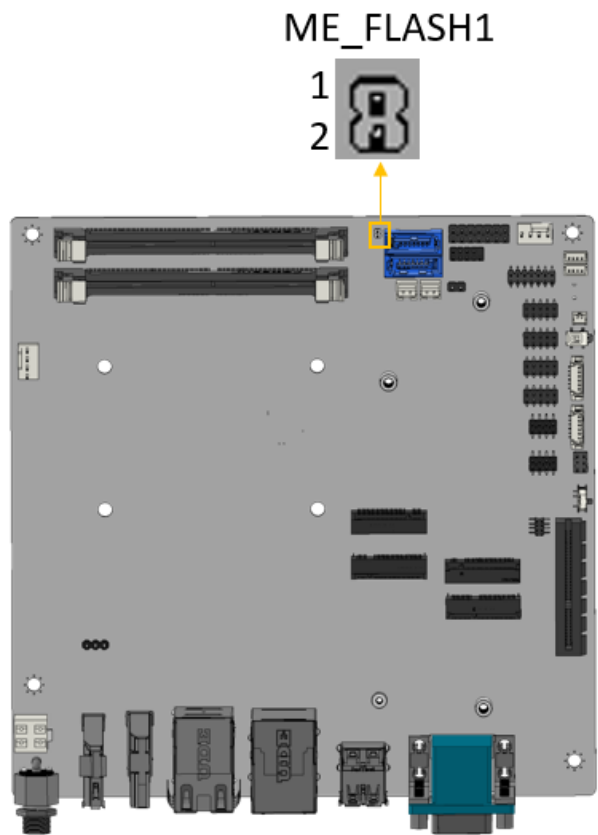
Figure 3-5: Flash Descriptor Override Setting Jumper Locations
