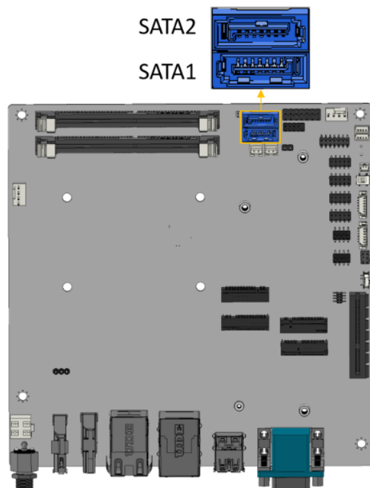
Figure 3-14: SATA 6Gb/s Drive Connectors Location
