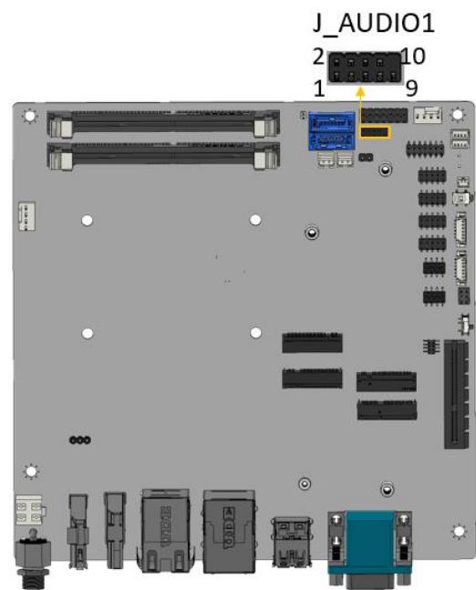
Figure 3-6: Audio Connector Location
