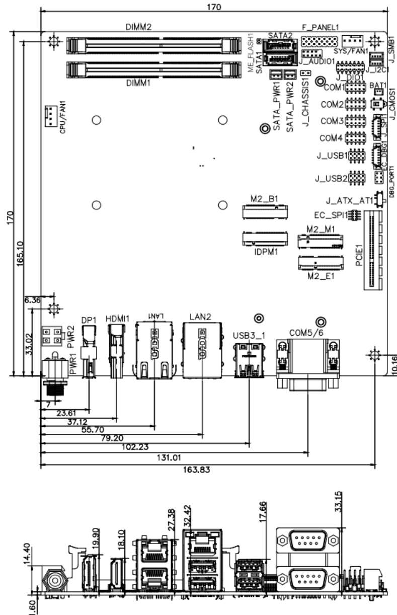
Figure 1-3: Dimensions (mm)
