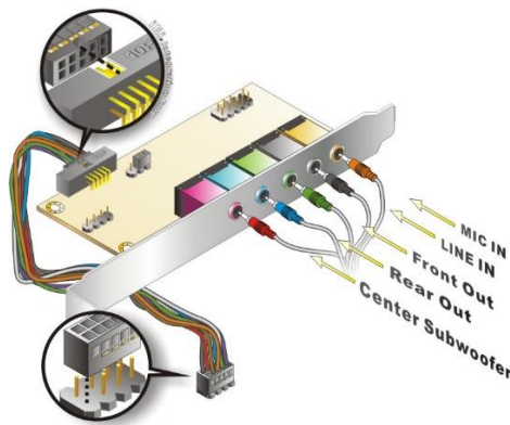
Figure 4-5: 7.1 Channel Audio Kit
