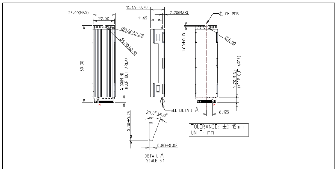
Figure 4: Innodisk M.2 (P80) 4IG2-P with heat-spreading copper layer diagram
