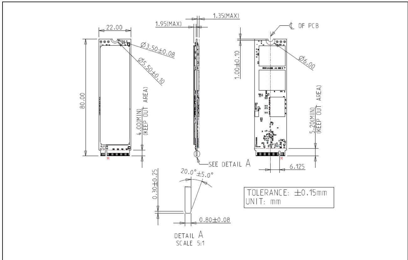
Figure 3: Innodisk M.2 (P80) 4IG2-P with heat-spreading copper layer diagram
