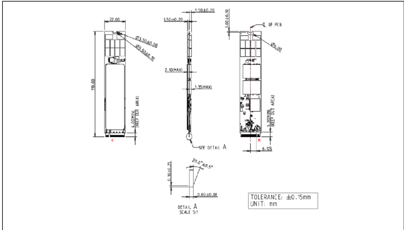
Figure 5: Innodisk M.2 (P110) 4IG2-P with heat-spreading copper layer diagram
