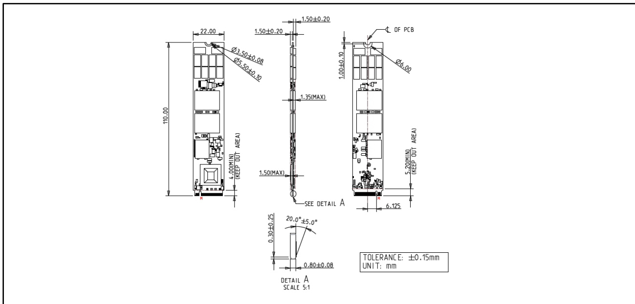
Figure 7: Innodisk M.2 (P110) 4IG2-P
