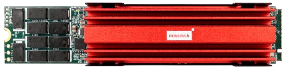
Figure 2: Innodisk M.2 (P110) 4IG2-P (Wide Temperature)
