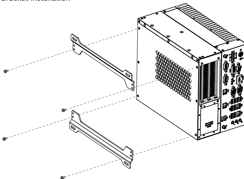
Wall mount bracket installation
