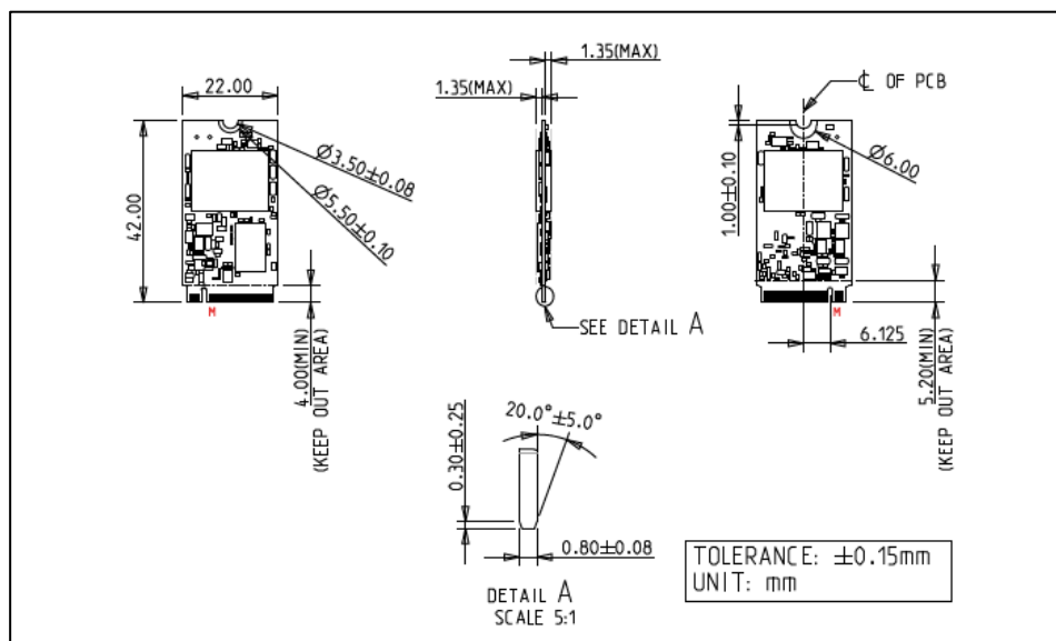
Figure 3: Innodisk M.2 (P42) 4IE3
