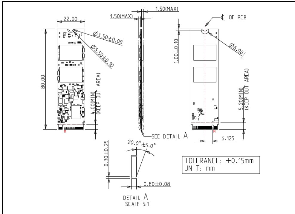
Figure 3: Innodisk M.2 (P80) 4IE3 mechanical drawing
