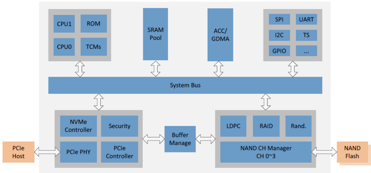
Figure 5: Innodisk M.2 (P80) 3IE8 Block Diagram
