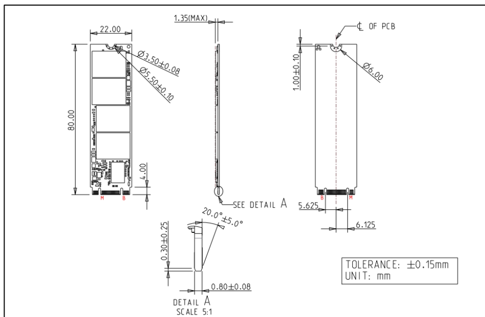
Figure 3: Innodisk M.2 (P80) 3IE8 diagram
