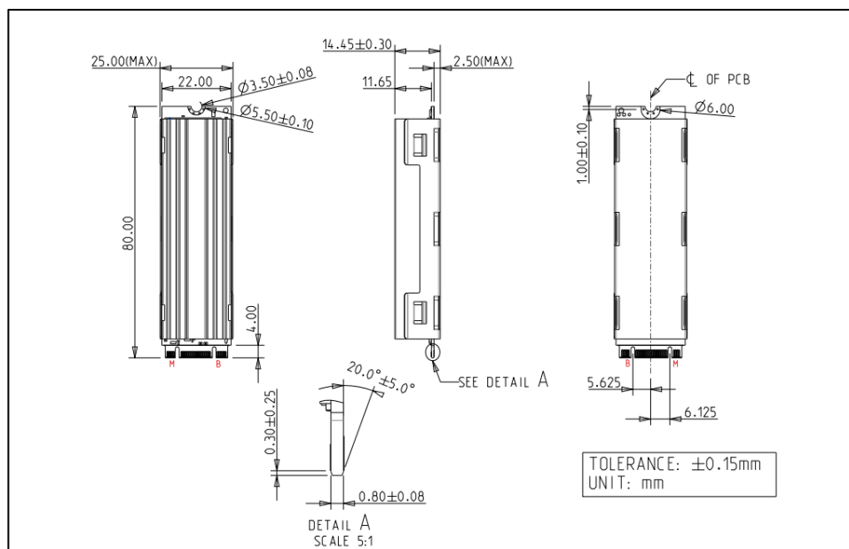
Figure 4: Innodisk M.2 (P80) 3IE8 with heatsink diagram
