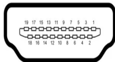
* Figure 4.4-2 HDMI Interface
