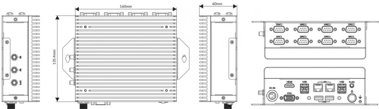
* Figure 3.2-1 NBC-2360 dimensional drawing
