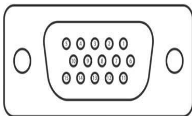
* Figure 4.4-1 VGA Interface
