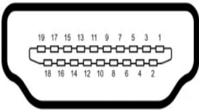
* Figure 4.5-2 HDMI Interface
