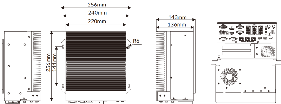
* Figure 3.2-1 MIC-8411 dimensional drawing
