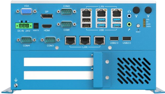
* Figure 4.1-1 MIC-8411 panel diagram
