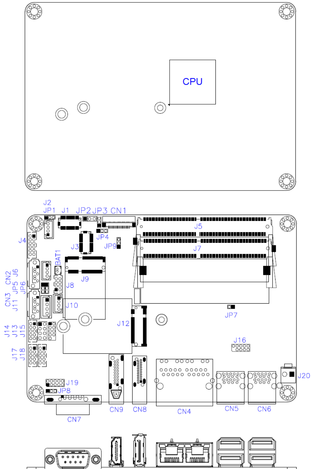
Board diagram of IB822
