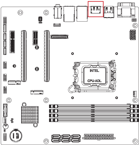
DP Connector
