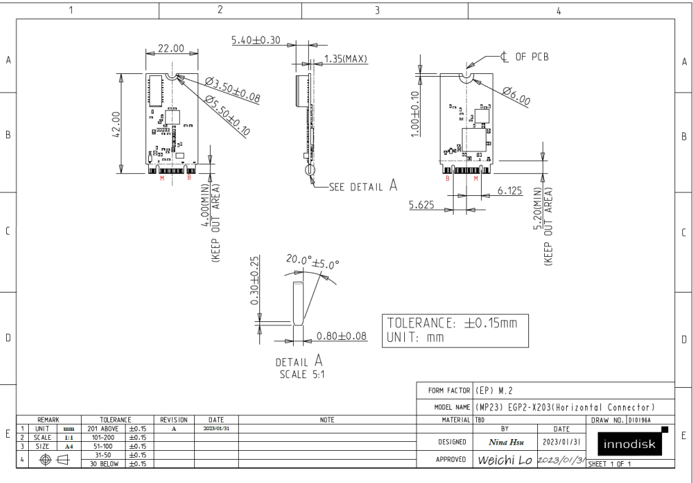
Figure 7: EGP2-X203-W2 Drawing
