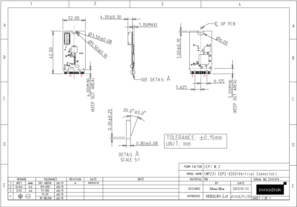
Figure 6: EGP2-X203-W1 Drawing
