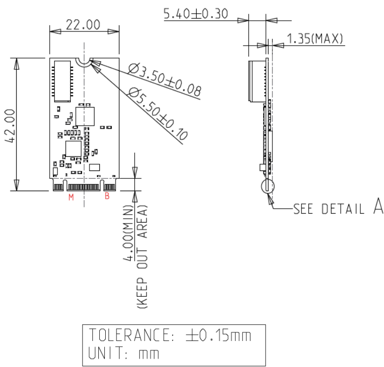
EGP2-X204-W2 (Horizontal Connector)
