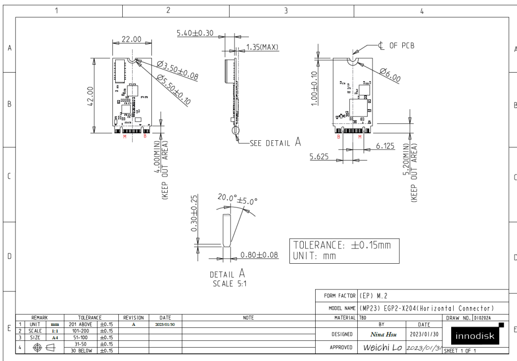
Figure 7: EGP2-X204-W2 Drawing
