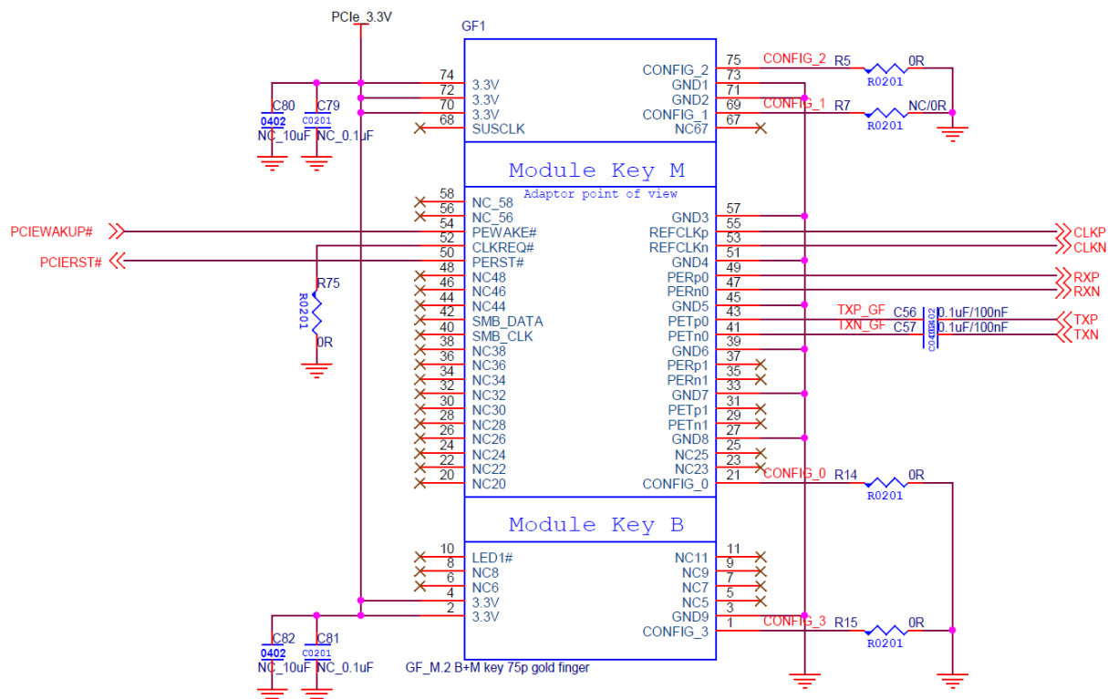
Figure 3: M.2 B-M Key Pin Define
