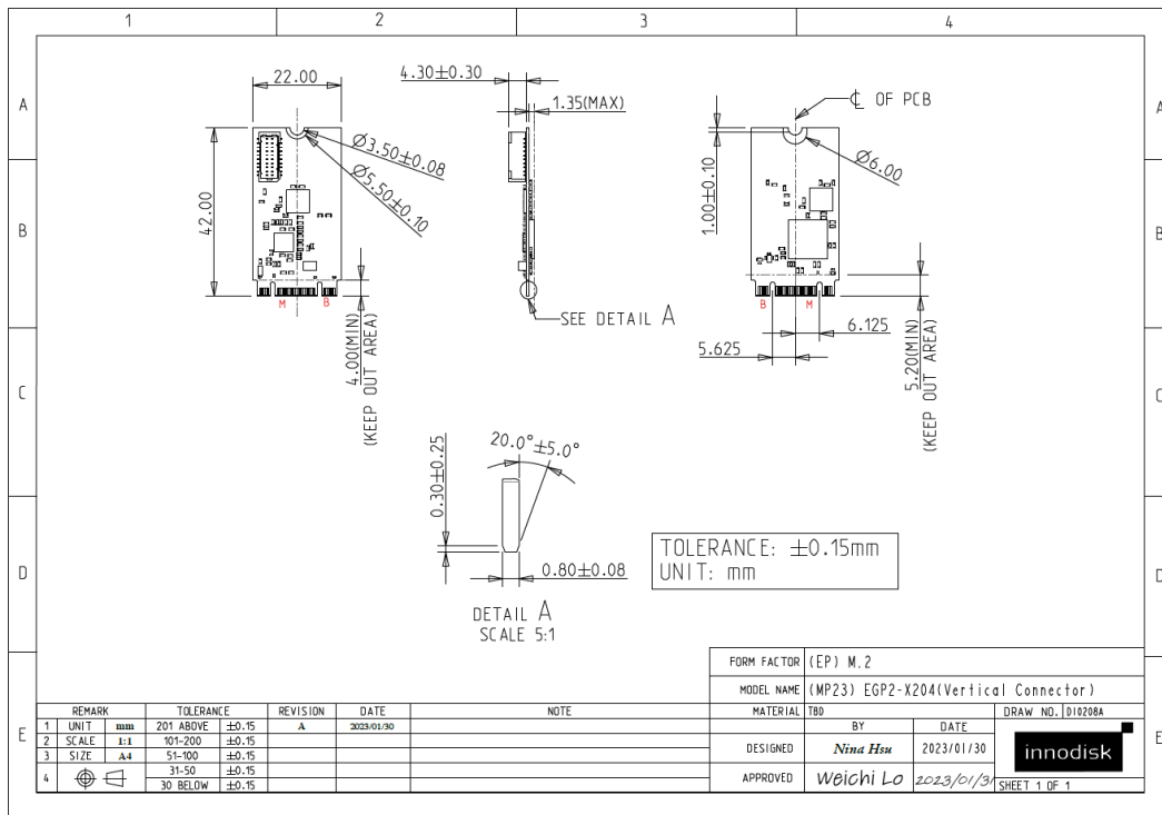
Figure 6: EGP2-X204-W1 Drawing
