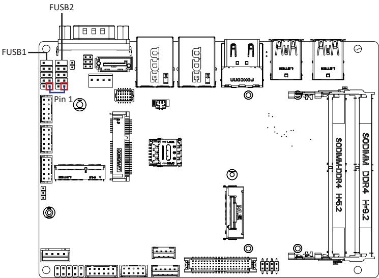
USB 2.0 Header
