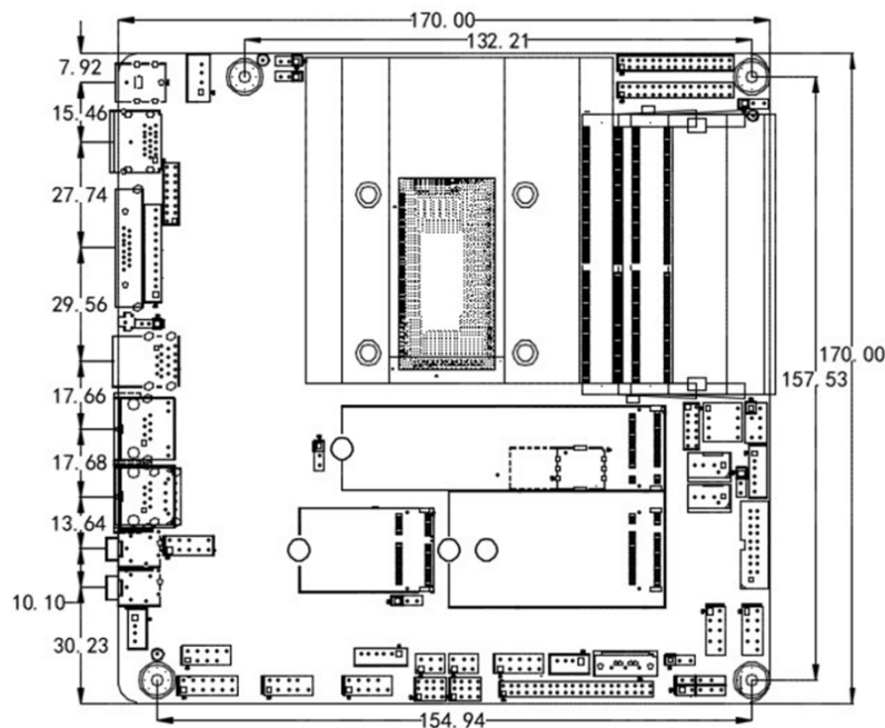
Figure 1 3.2 Main board size diagram
