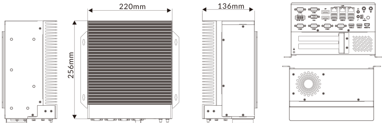
* Figure 3.2-1 MIC-7111 dimensional drawing
